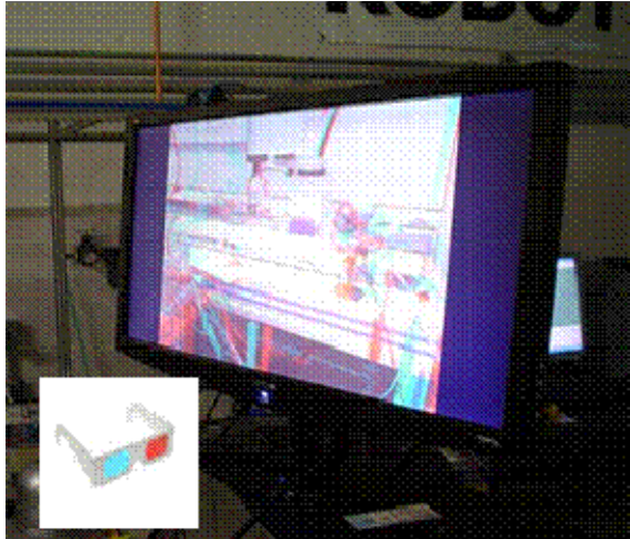
Figure 7: Anaglyph Video.
