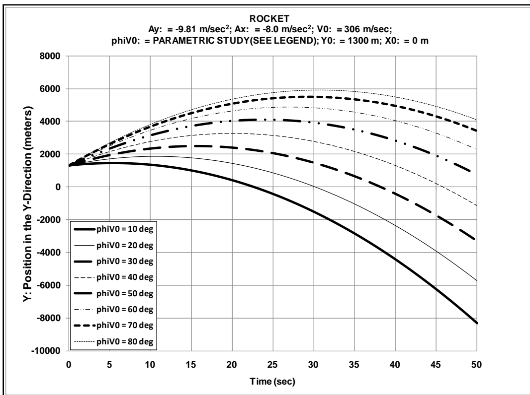
Figure 8. \underline{Y}(t) : Parametric Study of the Initial Velocity Angle ( \phi_{V0} ) From 10^\circ to 80^\circ .
