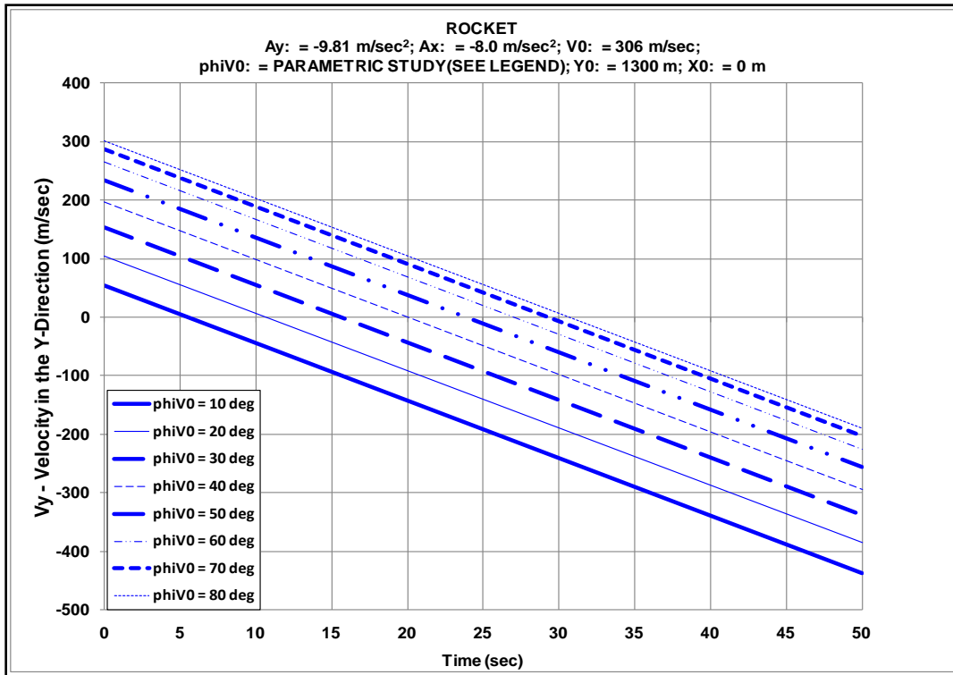
Figure 7. \underline{V}_y(t) : Parametric Study of the Initial Velocity Angle ( \phi_{V0} ) From 10^\circ to 80^\circ .
