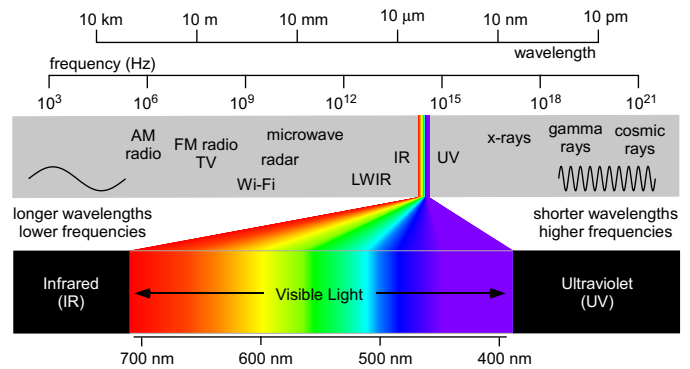
Fig. 1: Regions of the electromagnetic spectrum pertinent to this discussion.
