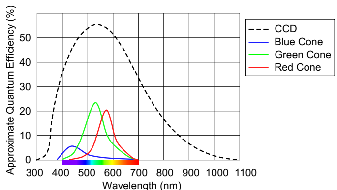
Fig. 2: Comparison of a typical silicon-based image sensor to human photoreceptors.
