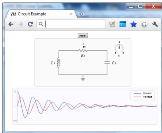
Figure 9: Electrical system.
