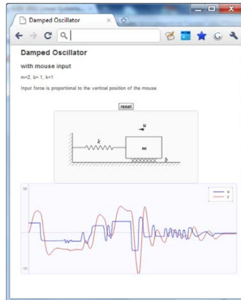
Figure 8: Input determined by mouse.
